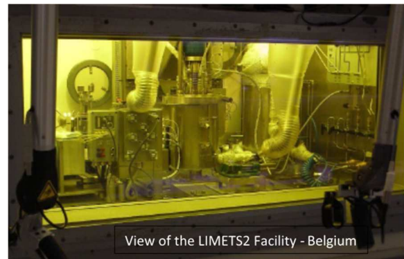
Figure IV-1: The LIMETS2 facility (SCK-CEN, Belgium)
