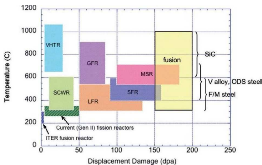
Figure IX-1: Requirements on materials in future Nuclear Energy Systems, Note: F/M = ferritic/martensitic; GFR = Gas Fast Reactor; ITER = International Thermonuclear Experimental Reactor; LFR = Lead Fast Reactor; MSR = Molten Salt Reactor; ODS = Oxide Dispersion Strengthened; SCWR = SuperCritical Water Reactor; SFR = Sodium Fast Reactor; VHTR = Very High Temperature Reactor.
