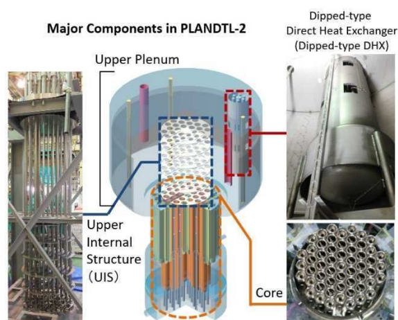
Figure III-5: The PLANDTL-2 facility at O Arai, Japan
