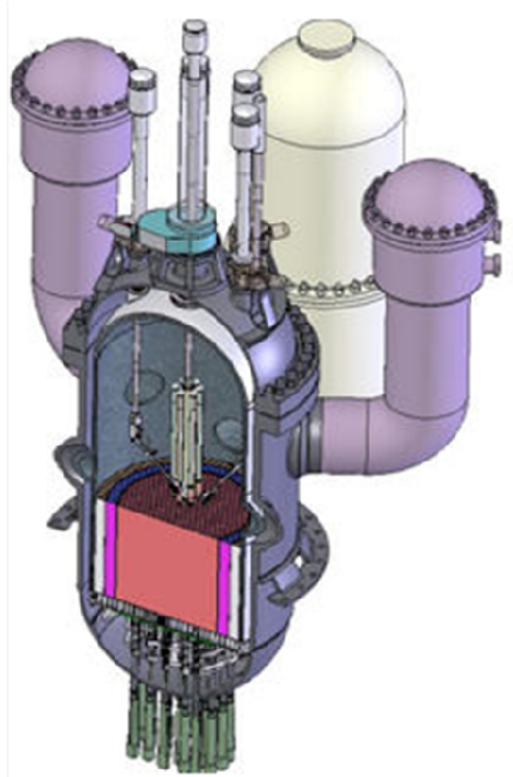
GFR - reactor, decay heat loops, main heat exchangers and fuel handling equipment
